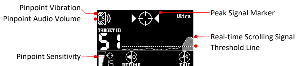
Pinpoint User Interface in Standard User Mode
