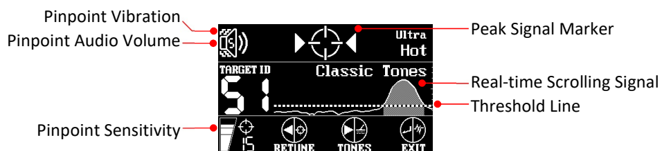
Pinpoint User Interface in Advanced User Mode
