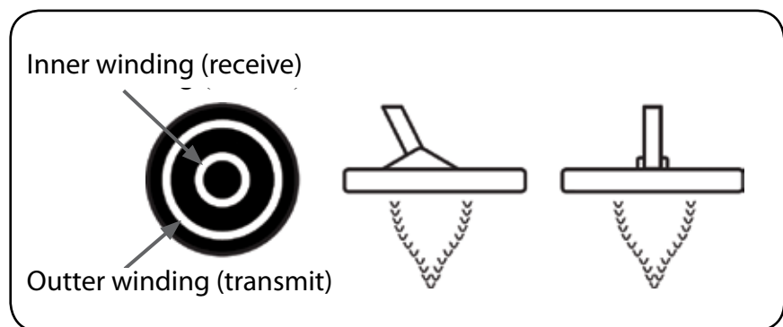
Concentric coil
