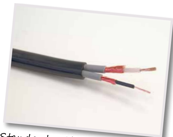
Standard cable contains more copper and is therefore heavier and more likely to be detected when bumped
